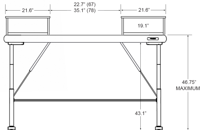
Quad Elevation 400 lbs lifting capacity*
