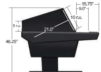
V Series profile with V1005 rack module.
