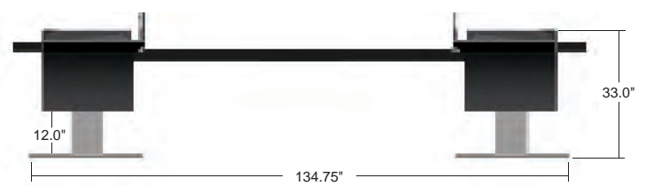
Mirage D-Control32 Dimensions
