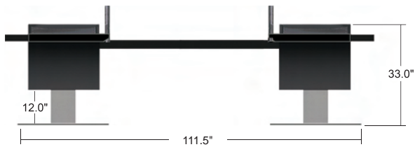
Mirage D-Control16 Dimensions
