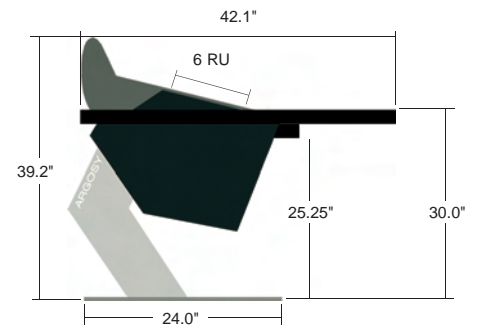
Mirage D-Control Dimensions
